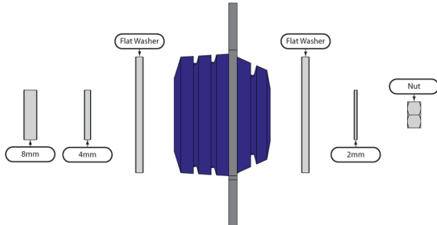
-1/4° Caster Change
