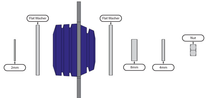
+1° Caster Change
