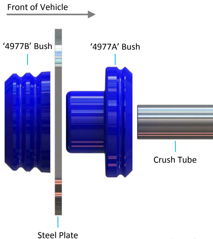
Figure 01 – Bush Installation
