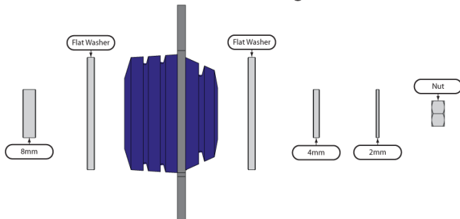
+1/4° Caster Change
