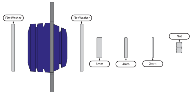
+1 1/4° Caster Change
