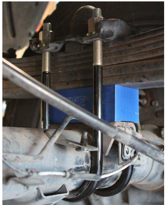
Picture 4: U-bolt tightened
