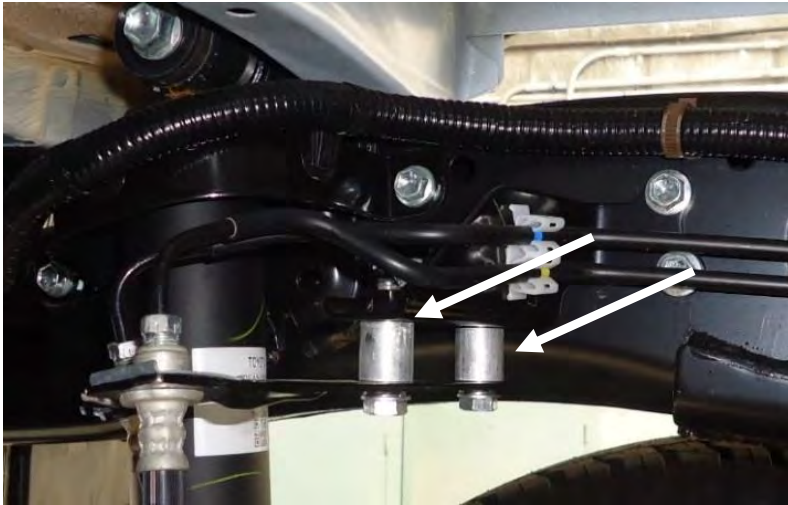
Picture 2: Rear upper brake hose mount spacer position
