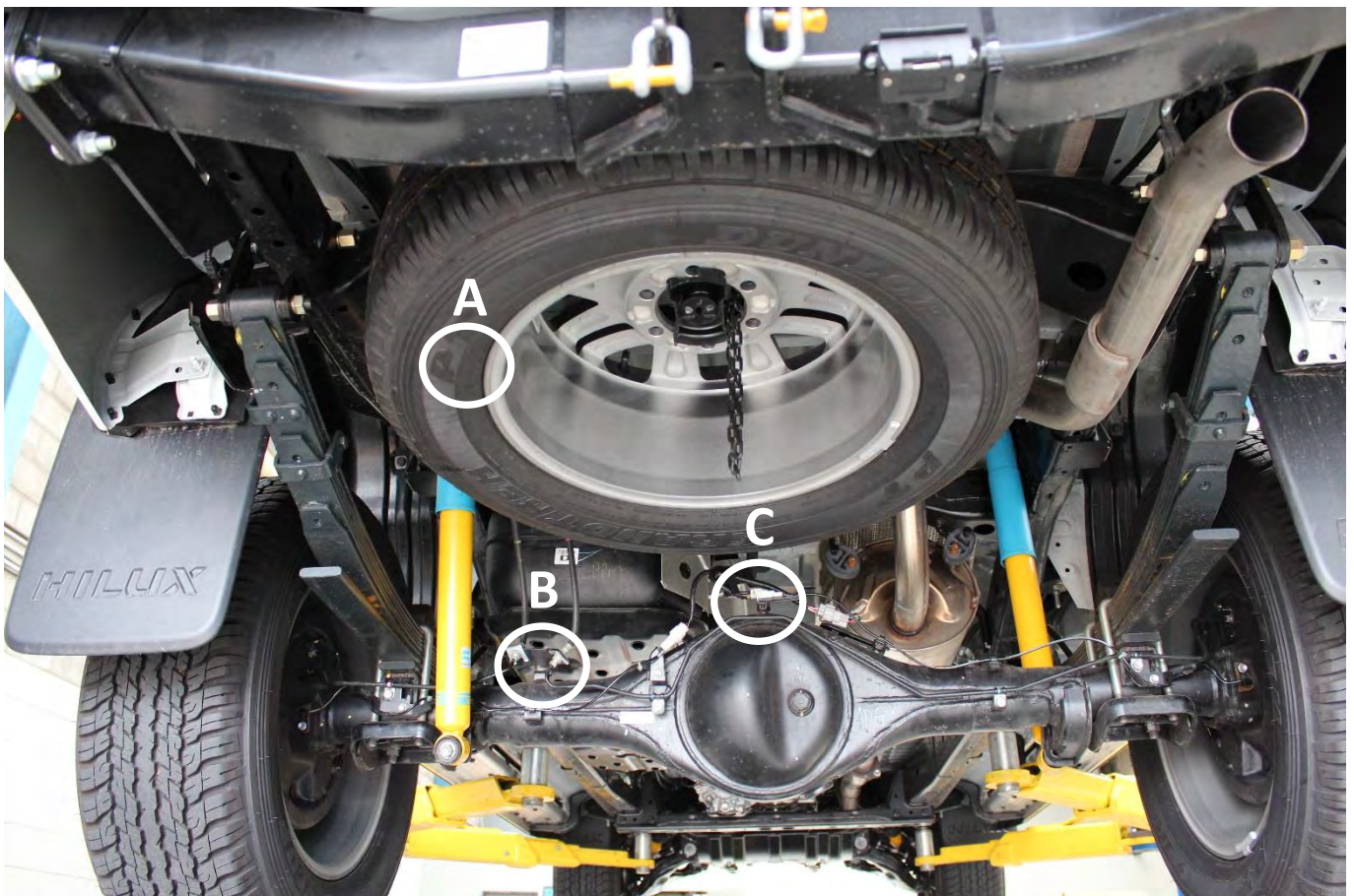
Picture 1: Underneath view of Hilux rear axle
