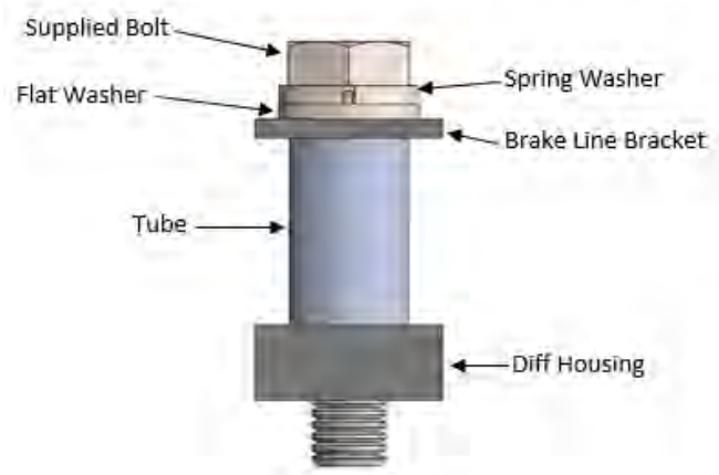
Picture 5: Assembly of brake hose mount spacer
